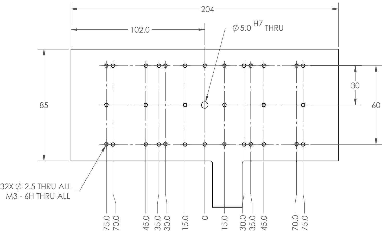
CARRIAGE MOUNTING DIMENSIONS
